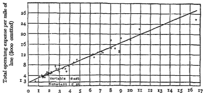
FIG 2—Gross ton miles per mile of line (100,000 omitted)
